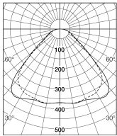
Delta 300x600
